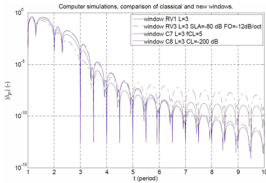
Fig. 9. Influence of the window on the power estimation bias for various windows.
