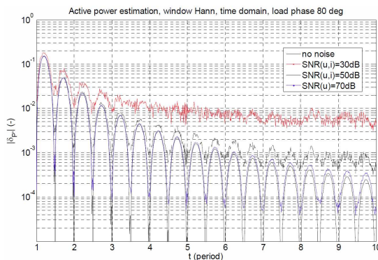
Fig. 5. Example of the influence of the additive noise of the input signals on the active power relative bias for a signal without noise and for SNR 70 dB, 50 dB and 30 dB, computer simulations.
