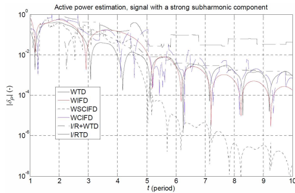
Fig. 4. Dependence of the relative bias of active power estimation for the investigated methods on sampling time. The signal is composed of a fundamental harmonic component and a sub-harmonic component.
